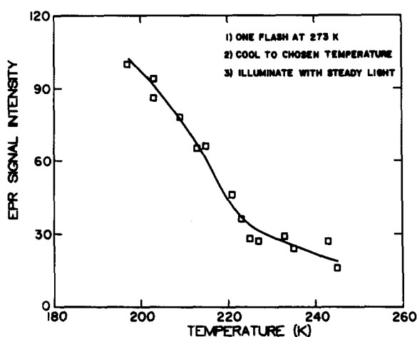
Fig. 4. Amplitude of the multiline signal produced in broken chloroplasts by a single flash at 273 K followed by continuous illumination at different temperatures. Samples were given an intense flash at 273 K, frozen in liquid nitrogen, then warmed to the specified temperature at which they received 30 s of continuous illumination. Spectrometer conditions and signal amplitude determinations as in Fig. 1.
