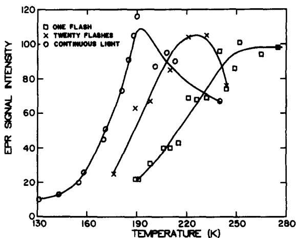
Fig. 3. Amplitude of the multiline signal produced by a single flash ( \square ), 20 flashes ( \times ), and 30 s continuous light ( \circ ) at different temperatures. The signal amplitudes for different illumination schemes have been separately normalized. Spectrometer conditions and signal amplitude determinations as in Fig. 1.
