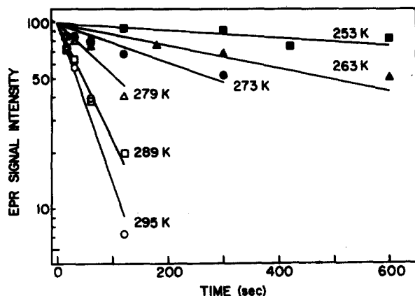
Fig. 1. Decay of the multiline signal amplitude at different temperatures. Broken chloroplasts were given one flash at the specified temperature, then placed in liquid N_2 after a variable delay. The signal amplitudes were taken as the peak-to-peak height of four lines downfield from g = 2 . The amplitudes at each temperature are normalized to the maximum value. Spectrometer conditions: microwave power, 50 mW; microwave frequency, 9.2 GHz; modulation amplitude, 32 G; modulation frequency, 100 kHz; temperature, 10 K.
