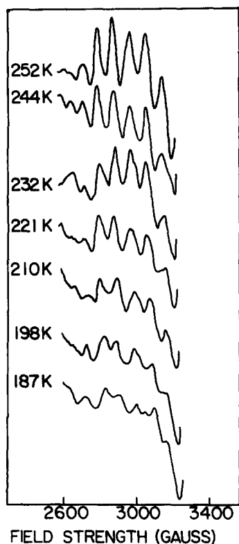
Fig. 2. Production of the multiline signal in broken chloroplasts by a single flash at different temperatures. Spectrometer conditions as in Fig. 1.
